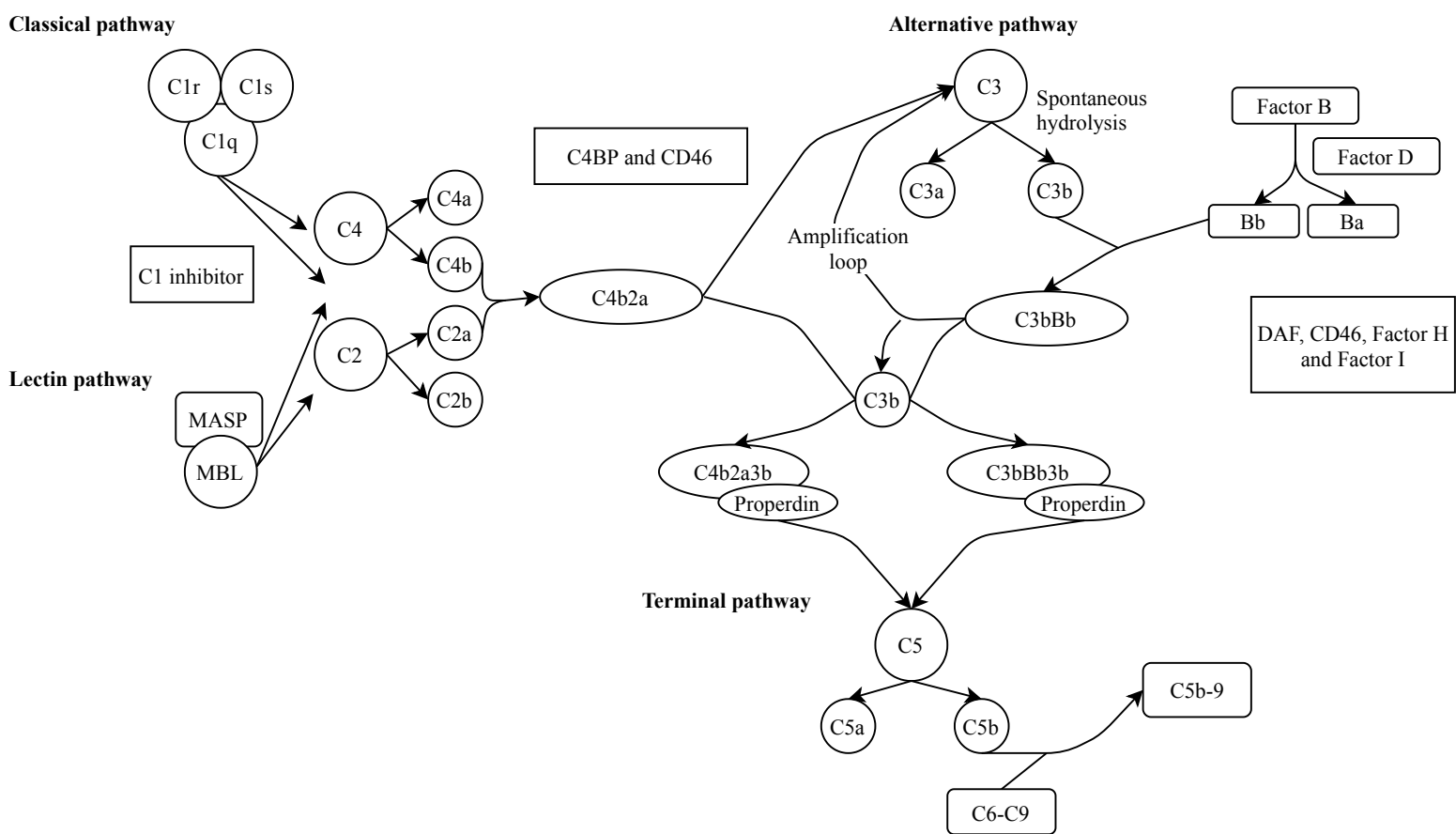
Fig. 1 Complement cascade
